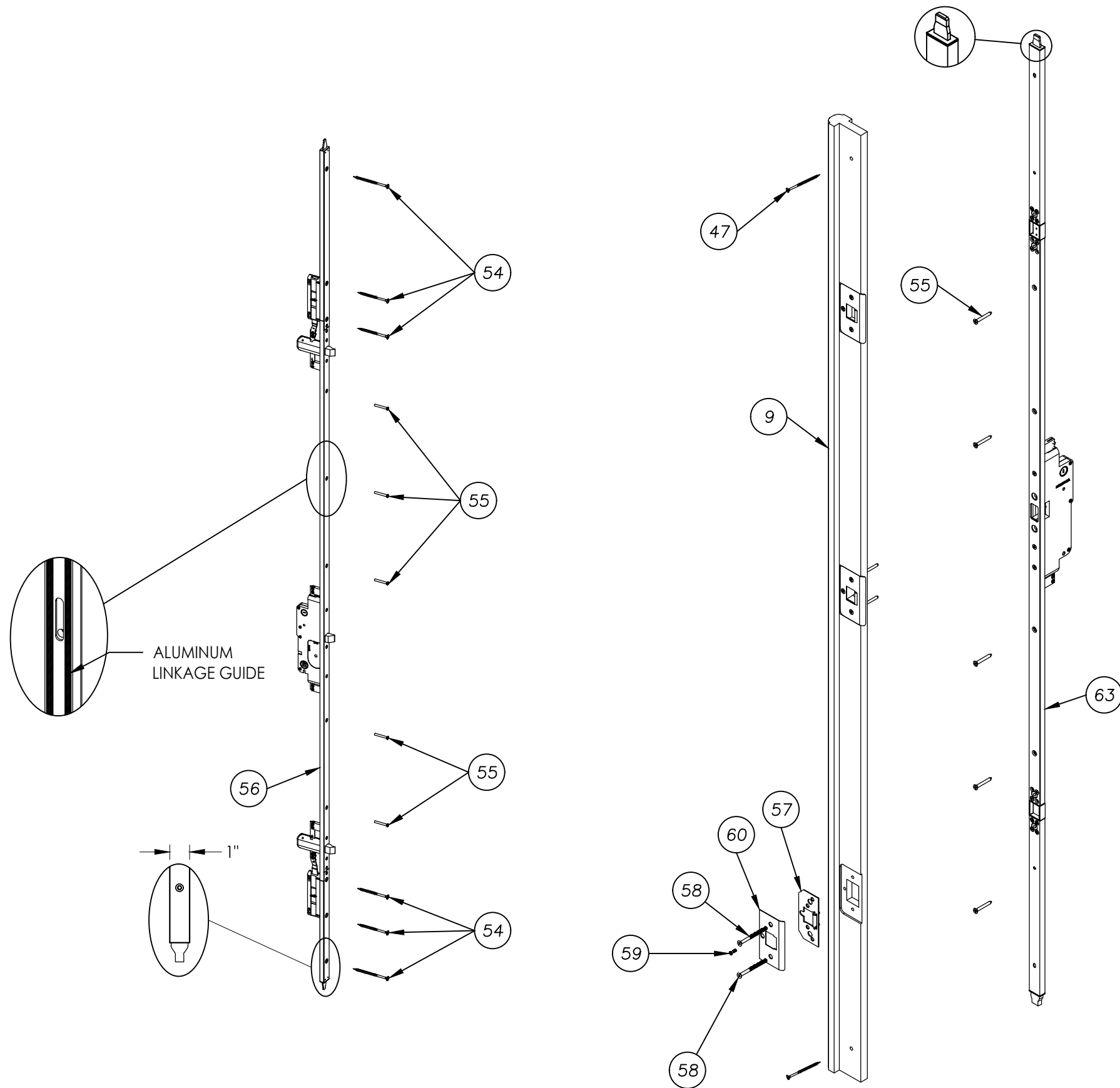
5 POINT LOCK
