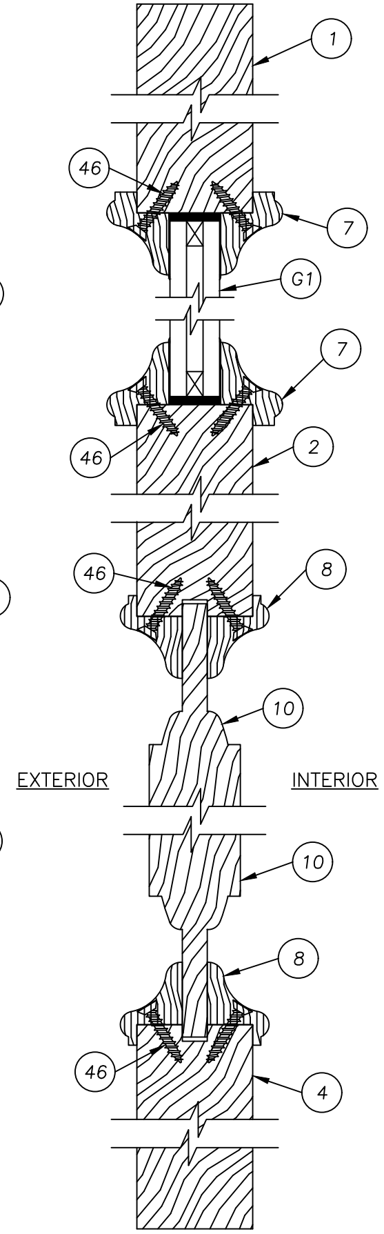
VERTICAL CROSS SECTION PANEL OVER PANEL
