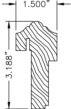
9 ASTRAGAL CAOBA
