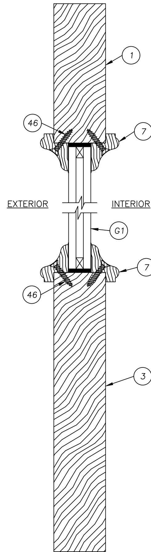
3 VERTICAL CROSS SECTION 2 FULL LITE PANEL
