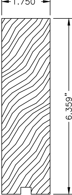
2 MIDRAIL CAOBA
